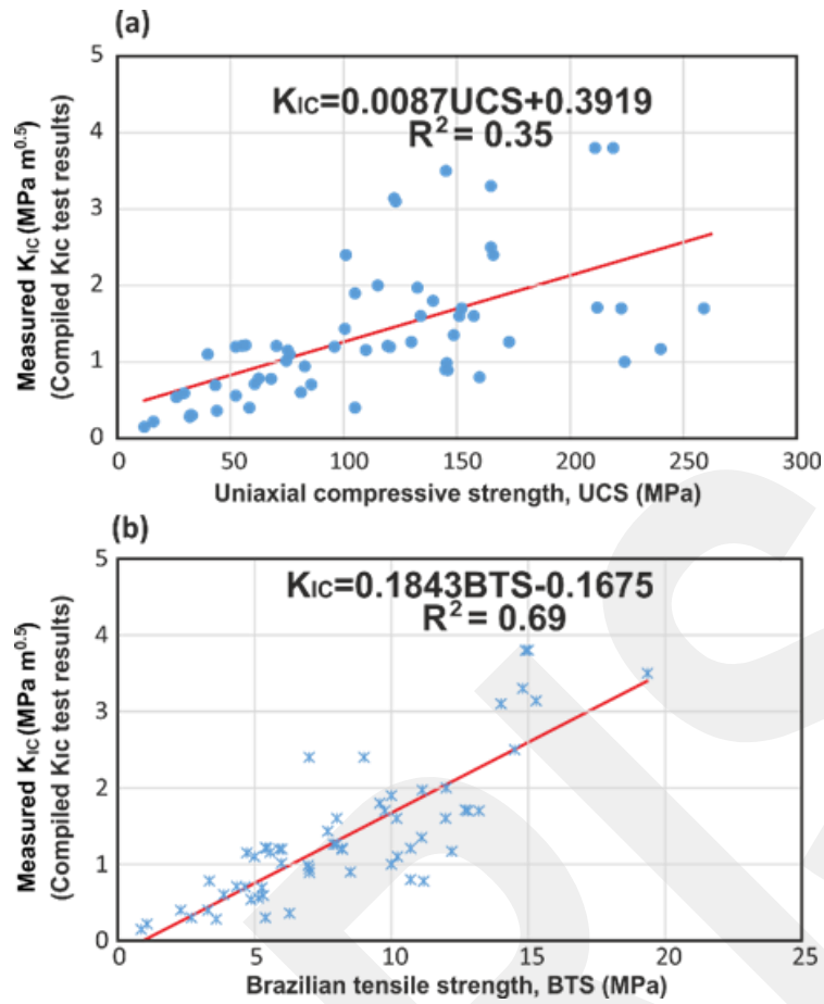
Figure 6. Simple regression models for the evaluation of K_{Ic} based on different rock properties a) UCS b) BTS
