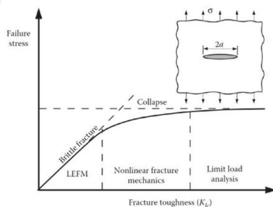
Figure 1. Effect of fracture toughness on the governing failure mechanism in a typical brittle material (LEFM: Linear elastic fracture mechanics, 2a : diameter of the crack plate, \sigma : tensile stress triggering fracture development) [2]
