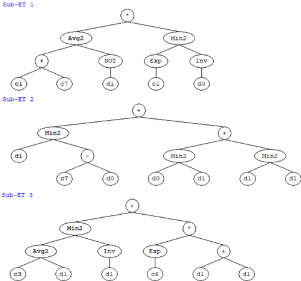
Figure 5. Sub-expression trees of the established GEP model (d0: UCS, d1: BTS, g1c1: -3.702, g1c7: 2.008, g2c7: -0.552, g3c3: -1.851, g3c6: -4.378)
