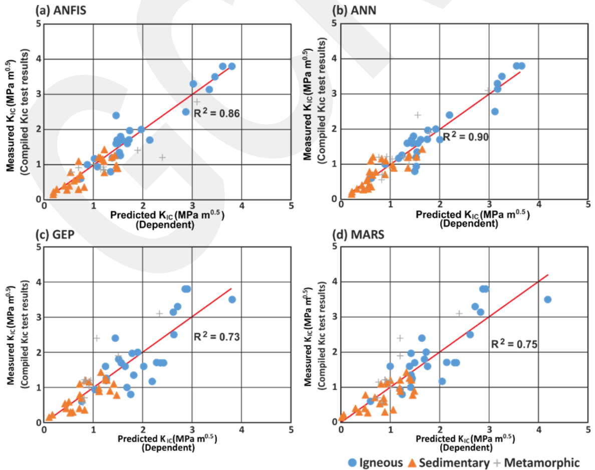
Figure 7. Predicted and measured K_{Ic} values for the established models a) ANFIS b) ANN c) GEP d) MARS
