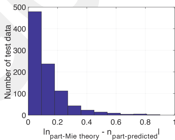
Figure 5.3 Histogram of the differences between actual and estimated particle refractive index for randomly selected 20% of the dataset.
