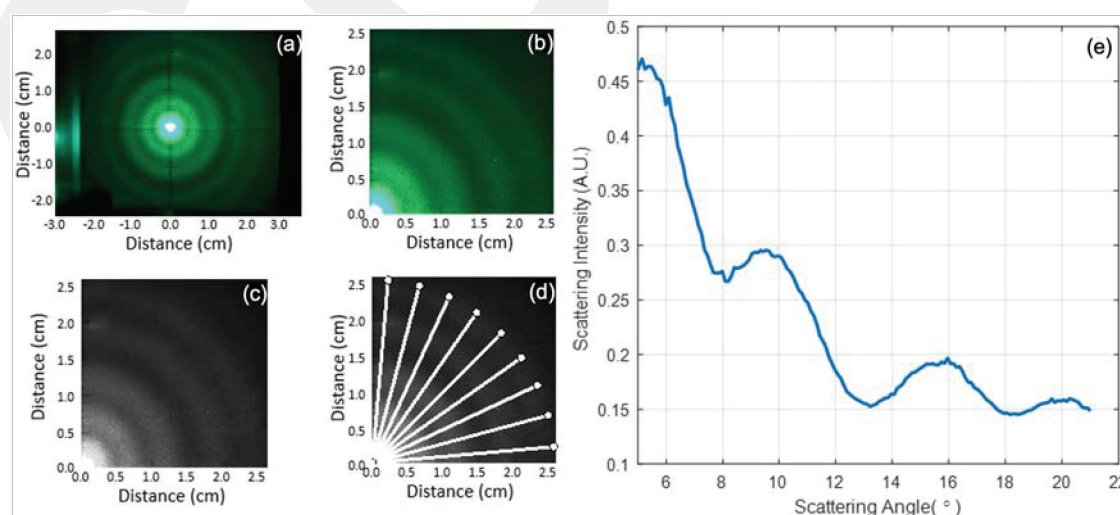
Figure 3.4 (a) Raw scattering image of Me8 particles excited by a green laser, (b) cropped image, (c) gray-scale image, (d) data lines on scattering image, (e) average scattering behavior of 86 lines (5°:1°:90°) on 1.50 fM 8 \mu m Me particles.
