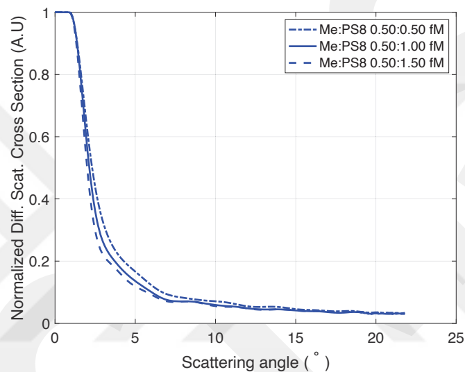
Figure 4.13 Scattering of Me8 and PS8 particles at 1:1 ratio for 0.50 fM Me8 with 0.50 fM PS8, 1.00 fM PS8, and 1.50 fM PS8 concentrations by blue light.
