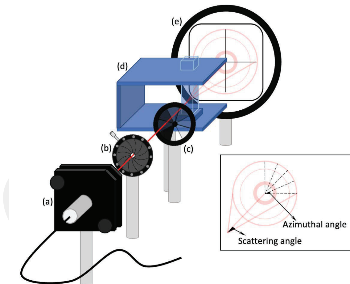
Figure 2.2 Illustration of the experimental setup, (a) light source, (b) iris, (c) neutral density filter, (d) cuvette holder and cuvette, and (e) graded white screen, (inset) azimuthal and scattering angles.
