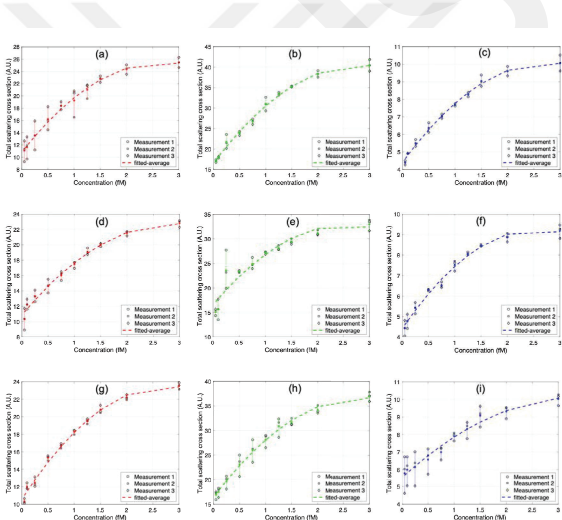
Figure 4.5 Total scattering intensity vs concentration change for Me8 (a, b, c), PS8 (d, e, f) and PS10 (g, h, i) materials by red, green, and blue lasers.
