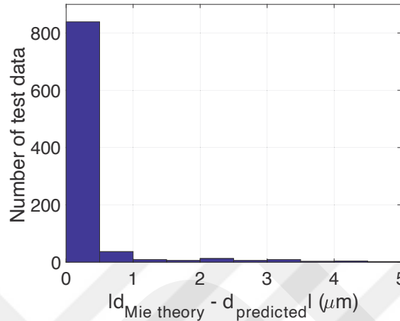
Figure 5.2 Histogram of the differences between actual and estimated particle size for randomly selected 20% of the dataset.
