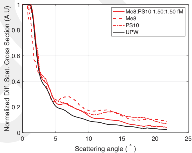
Figure 4.15 Scattering of Me8 and PS10 particles mixture at 1:1 ratio for 1.50 fM Me8 with 1.50 fM PS10 and ultra-pure water (UPW) by red light.
