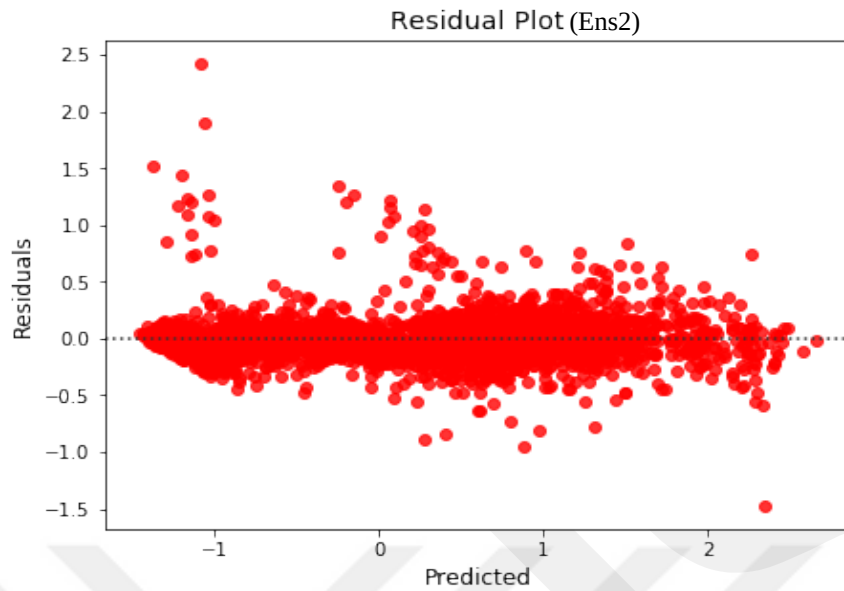
Figure 5.4 Residual Plots
