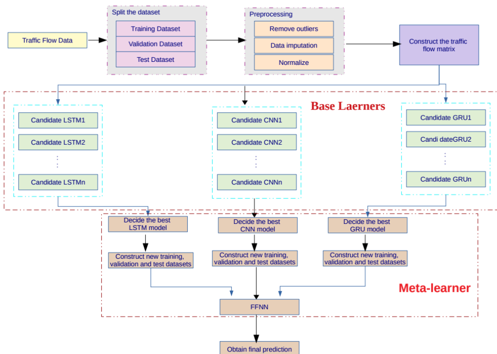
Figure 3.5 General structure of the alternative model.
