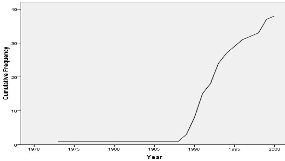
Figure 1. The cumulative increase of SBM adoptions by states: 1971 to 2000
