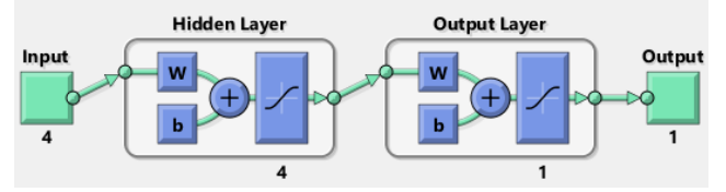
Fig 6. ANN architecture adopted in this study.
