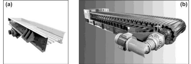
Fig 1. Typical feeders used in crushing-screening plants a) Grizzly feeder b) Apron feeder.
