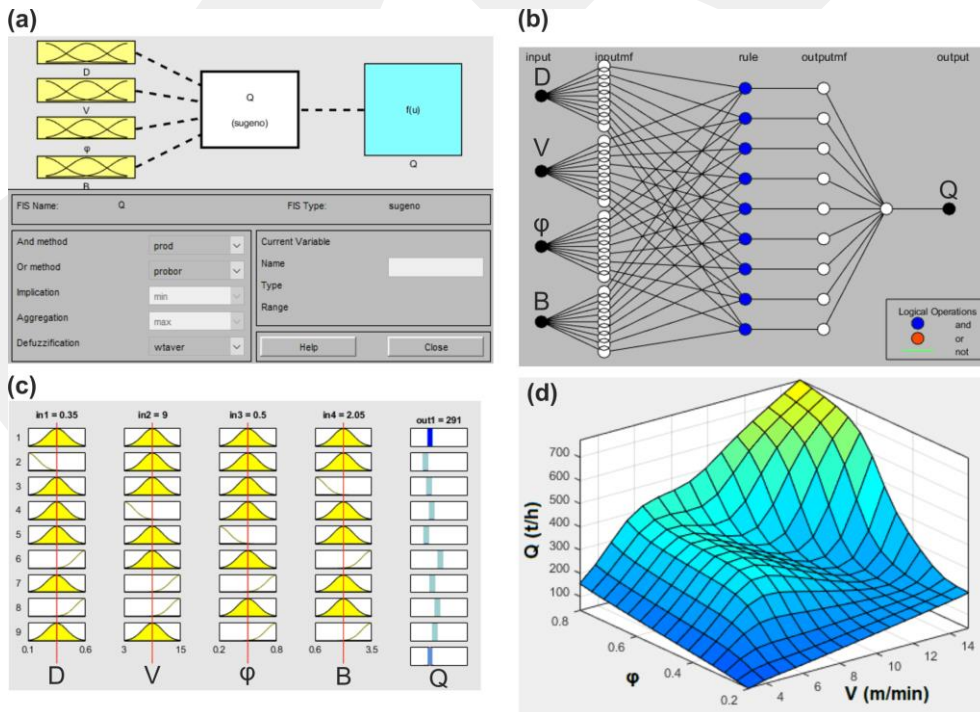
Fig 5. ANFIS outputs a) Input parameters b) ANFIS model structure c) Membership functions d) A typical surface plot based on \varphi and V.
