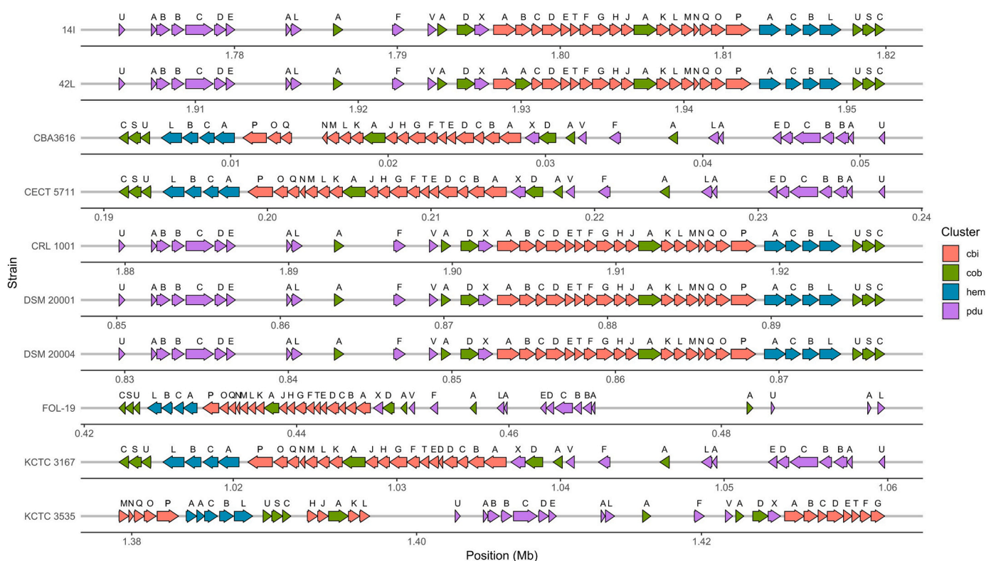
Fig. 7. Schematic representation of pdu and cbi-cob-hem clusters of ten L. coryniformis genomes.
