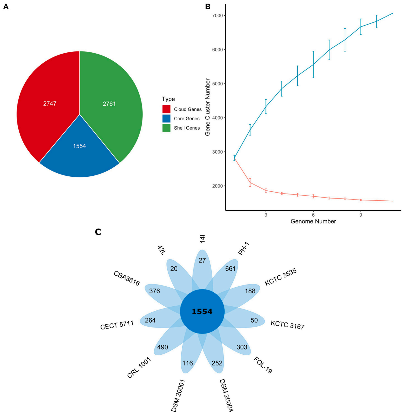
Fig. 3. (A) Coding sequence distributions in the eleven L. coryniformis pan-genome. Cloud genes (red), core genes (blue), and shell genes (green). (B) Estimation of core- (red line) and pan-genomes (blue line) of the eleven L. coryniformis strains by including genomes one by one. (C) Venn diagram representing the core and unique gene families of L. coryniformis obtained.
