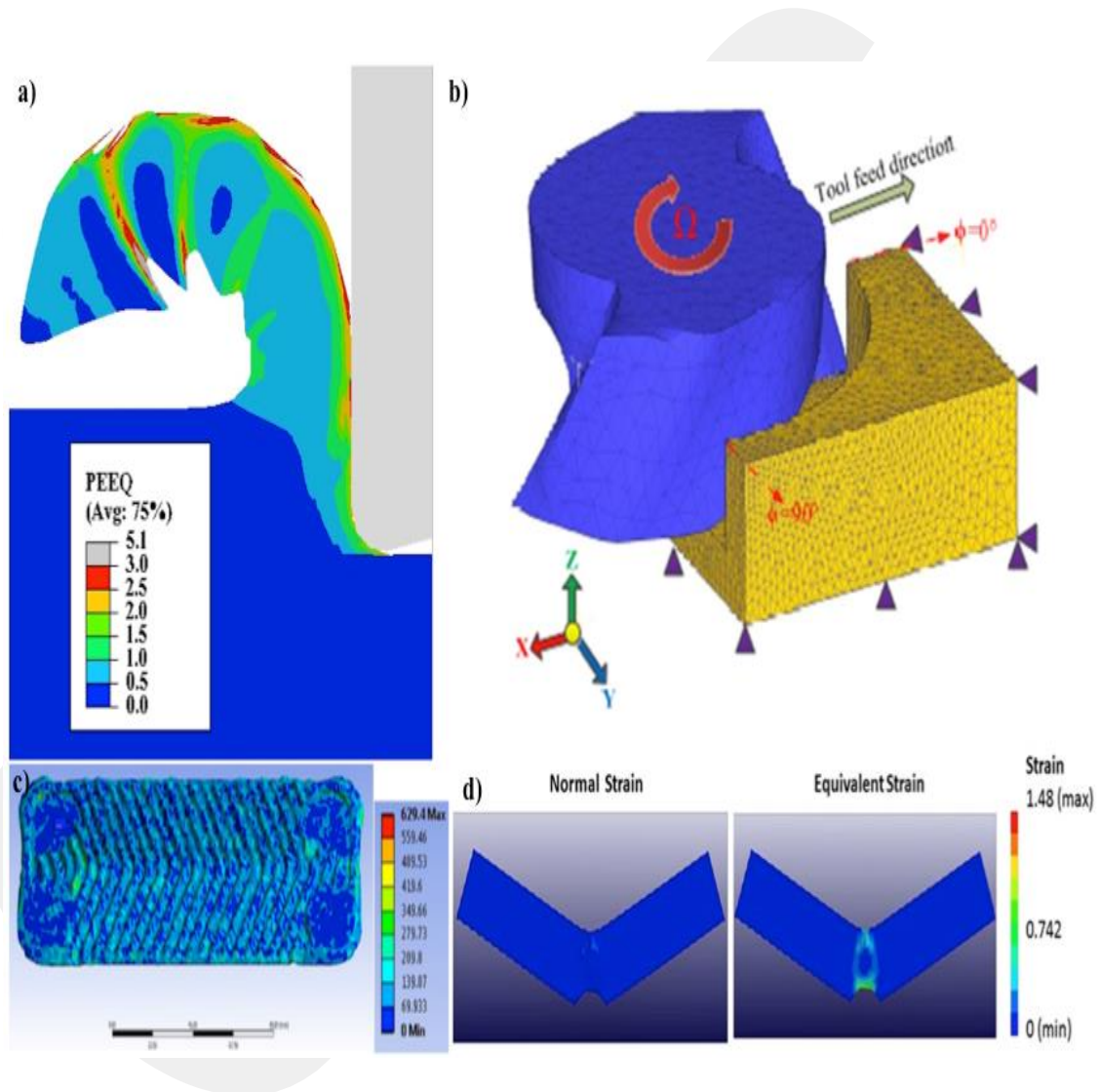
Figure 4.2.1 Examples of Finite Element Analysis a) the distribution of the equivalent plastic strain (PEEQ), of Ti-6Al-4V [29], b) 3-D FE model for half-immersion micro-end milling [46], c) Heterogeneous equivalent stress distribution on steel plate simulation [47], d) Demonstration of differences in normal and equivalent and strain fields upon a typical impact simulation of niobium-zirconium alloy [48]
