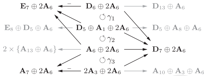
FIGURE 3. The graph \mathfrak{C}_7 .
