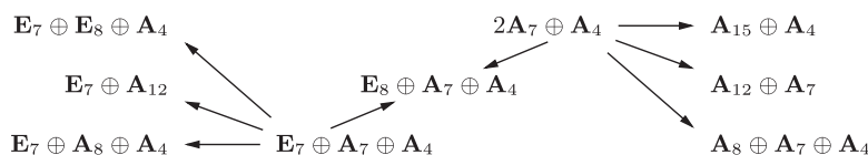
FIGURE 1. The graph \mathcal{C}_2 .
