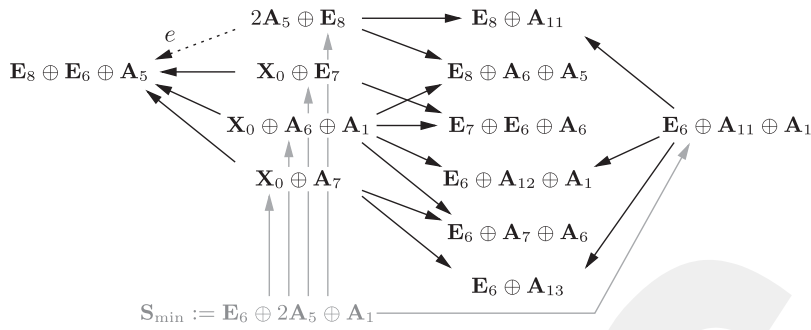
FIGURE 2. The graph \mathcal{C}_3 (where \mathbf{X}_0 := \mathbf{E}_6 \oplus \mathbf{A}_5 ).
