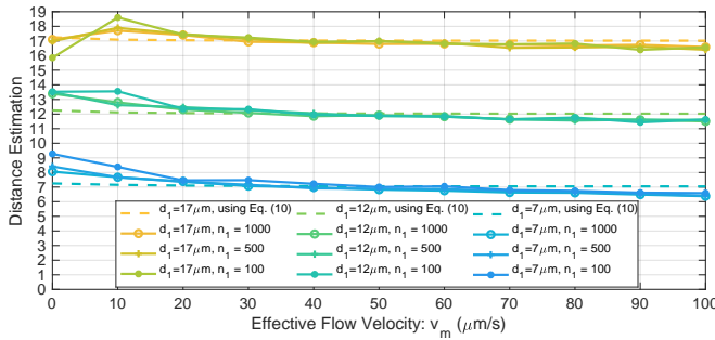
Fig. 4. Flow vs. distance estimation for two cases: (i) using t_{p,1} , which is the analytical peak time of the observed molecules (ii) using t_{p,1}^{\text{sim}} , which is the peak time obtained by particle-based simulations assuming that n_1 molecules are emitted ( D = 79.4 \mu\text{m}^2/\text{s} , r_v = 5 \mu\text{m} , w = 1 \mu\text{m} ).
