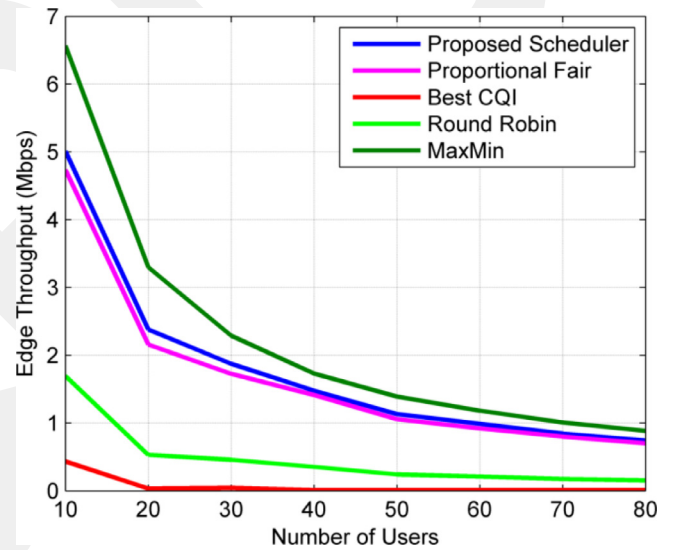
Fig. 4. Edge throughput performances of the schedulers.
