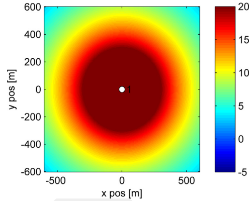
Fig. 19. SNR map, omnidirectional antenna, SISO.
