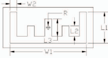
Figure 1. 5-fingers shaped microstrip patch antenna
