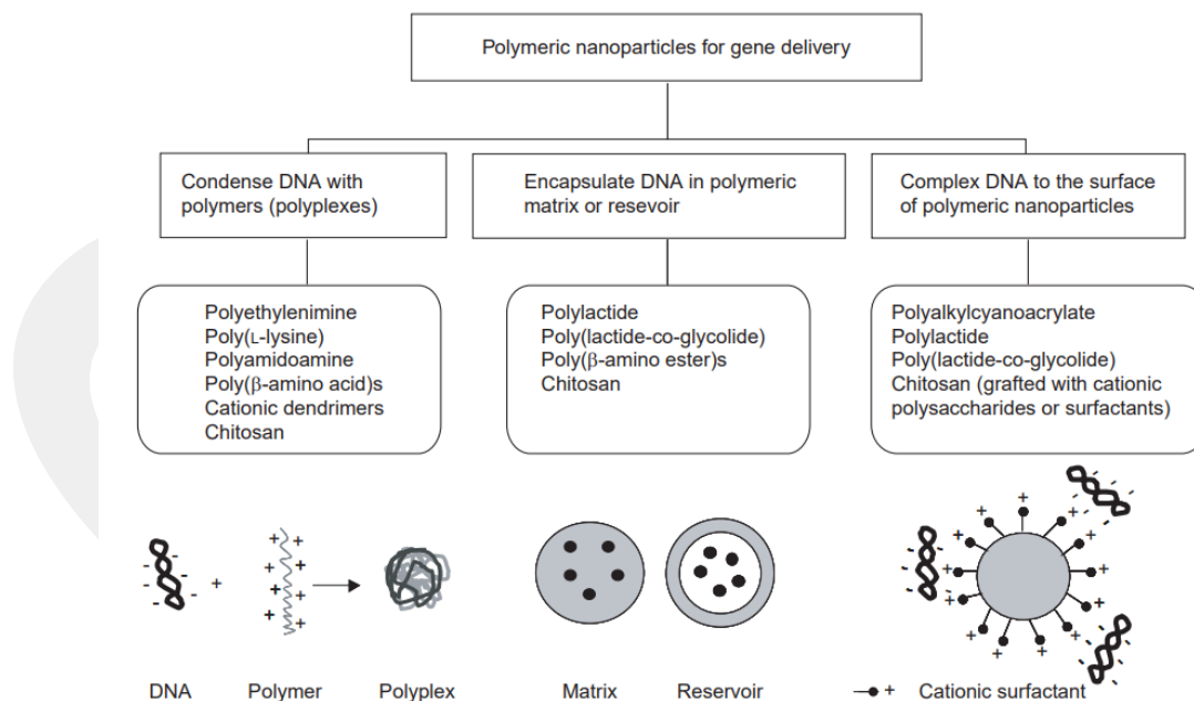
Figure 1.3. A schematic showing the different types of polymeric systems for gene delivery [24]
