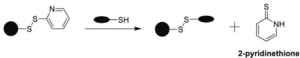
Figure 1.9. Schematic illustration for the replacement of the PD group by thiol-contained molecules [88]
