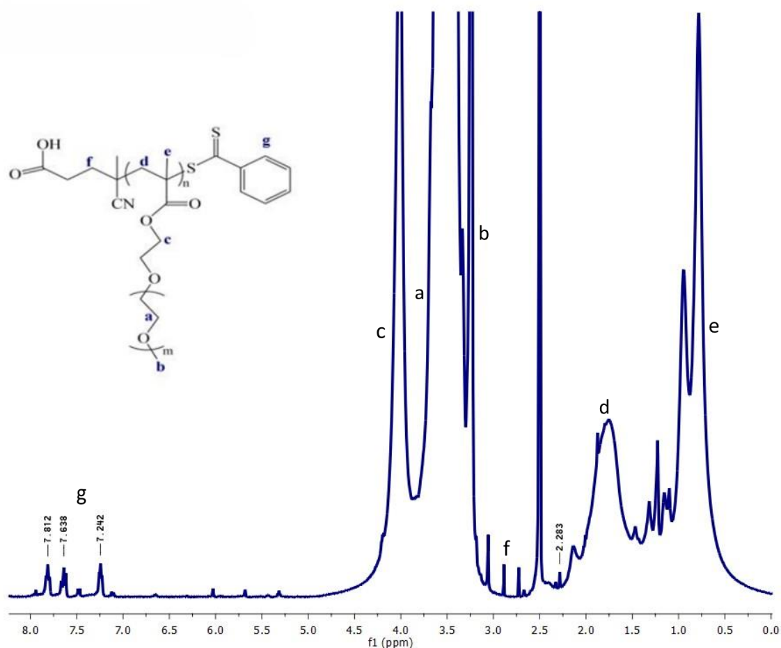
Figure 3.2. ^1\text{H} NMR spectra of POEGMA
