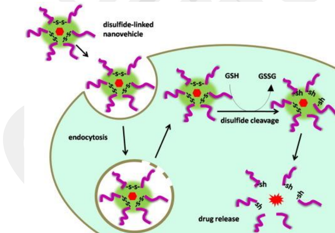
Figure 1.5. The mechanism of redox-sensitive nanocarriers for intracellular drug delivery [46]
