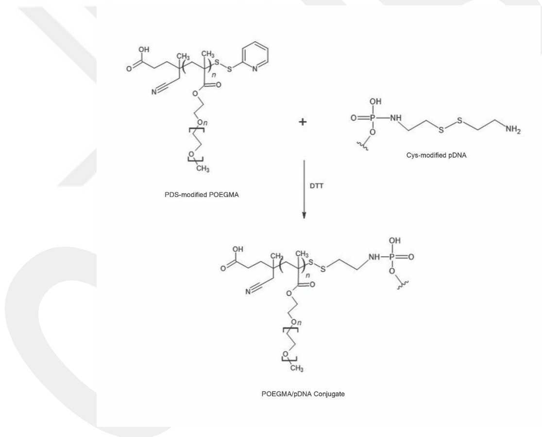
Figure 2.5. The Chemical Scheme for POEGMA and Plasmid Conjugation
