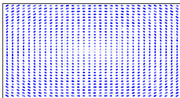
(c) 1024 QAM with Signal Generator (Lab Equipment)
