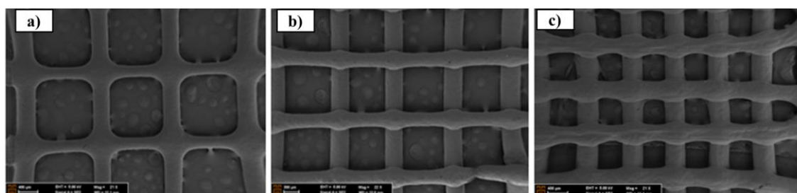
Figure 3.15 Evaluation of 50 PCL_Cf scaffolds in SEM; a) printed with 60% infill density, b) 80% infill density and c) 99% infill density. All scaffolds were printed in 5 mm/s and 206 kPa.
