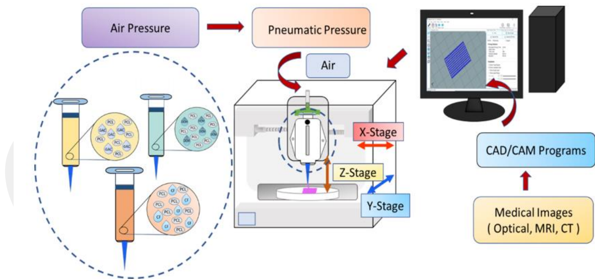
Figure 2.2 Representative image of a solution extrusion-based three-dimensional (3D) Bioprinter.
