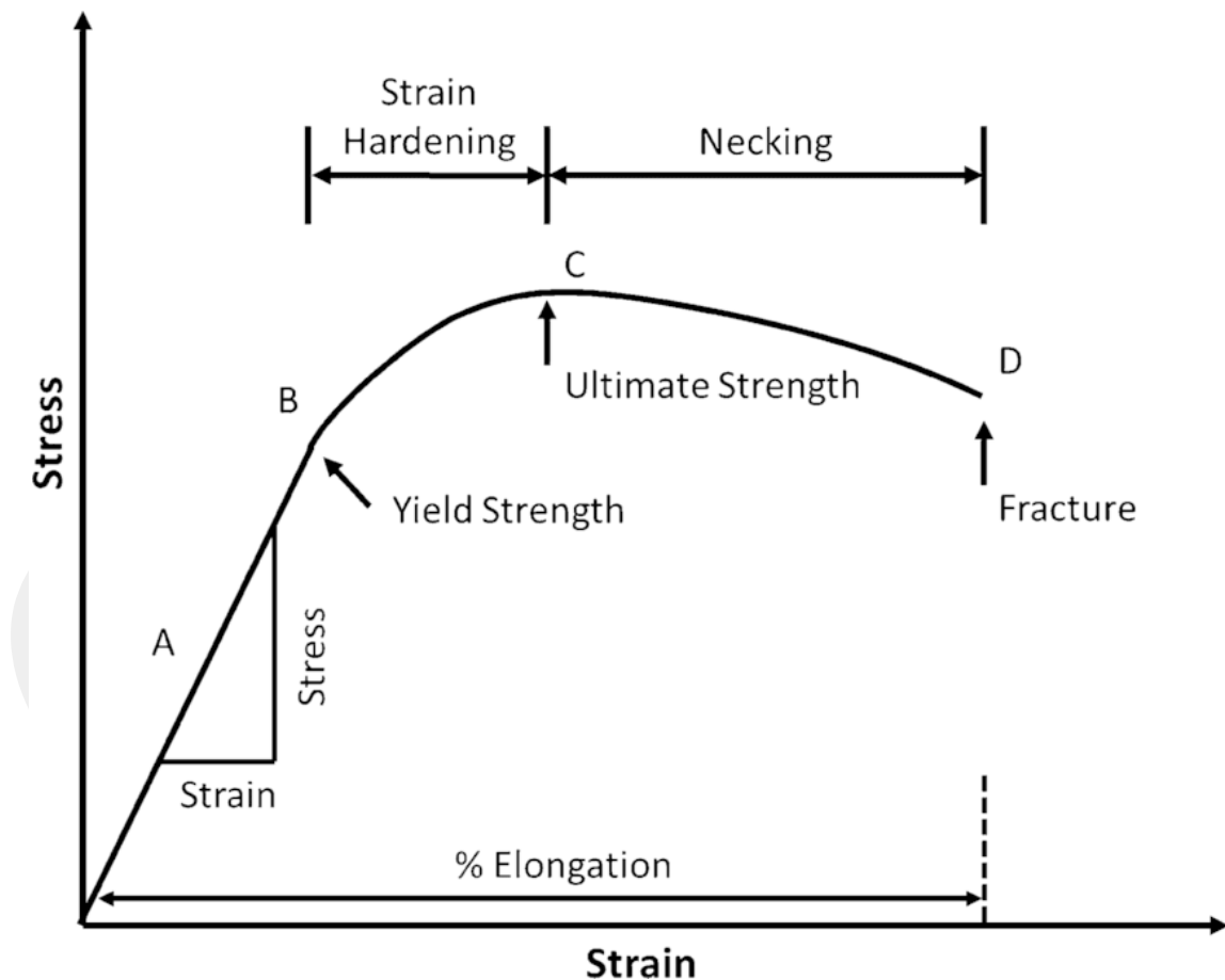
Figure 1.15 Stress-strain curve [96].
