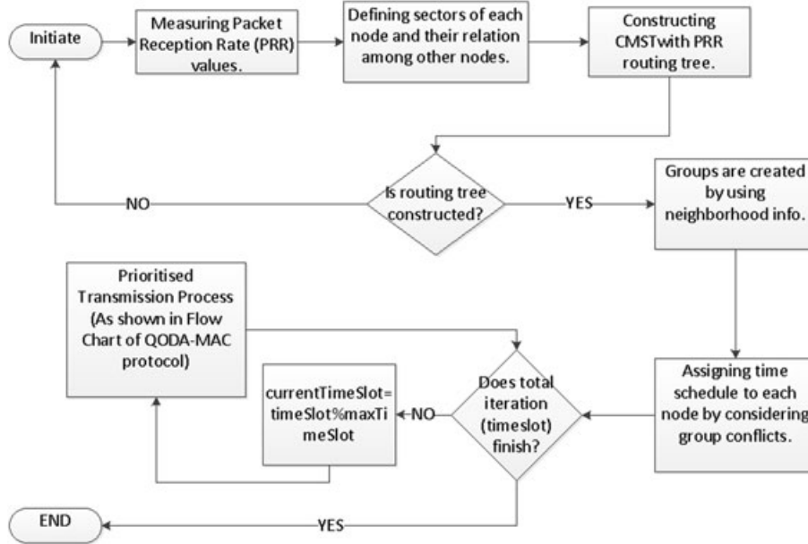
Figure 3. Flow chart of quality of service-aware four-sectored antenna-based medium access layer with service differentiation protocol.
