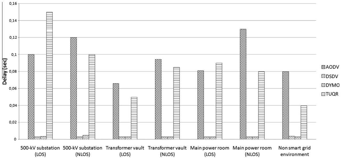
Fig. 4. Average network delay of AODV, DSDV, DYMO and TUQR routing protocols in different smart grid environments.
