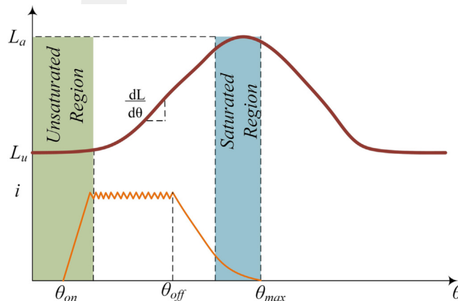
Fig. 3 Inductance and current profile of an SRM.
