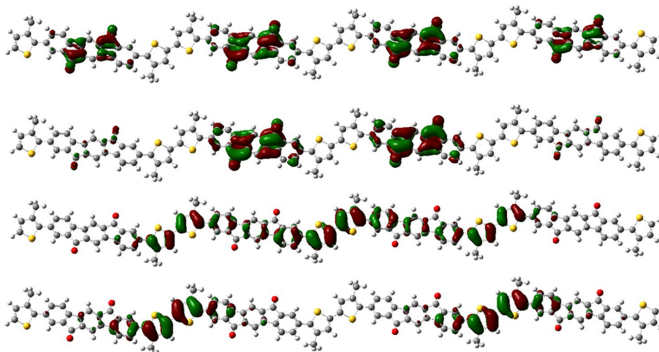
Fig. 7. – HOMO-1, HOMO, LUMO and LUMO + 1 (bottom to top) orbitals of 4-(IFDK-2T) . Partial localization of occupied orbitals on bithiophene and complete localization of unoccupied orbitals on indenofluorene units is clearly visible.
