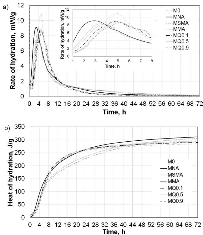
Fig. 6. a) Rate of hydration and b) heat of hydration of cementitious systems with variable PSD of anatase \text{TiO}_2 .
