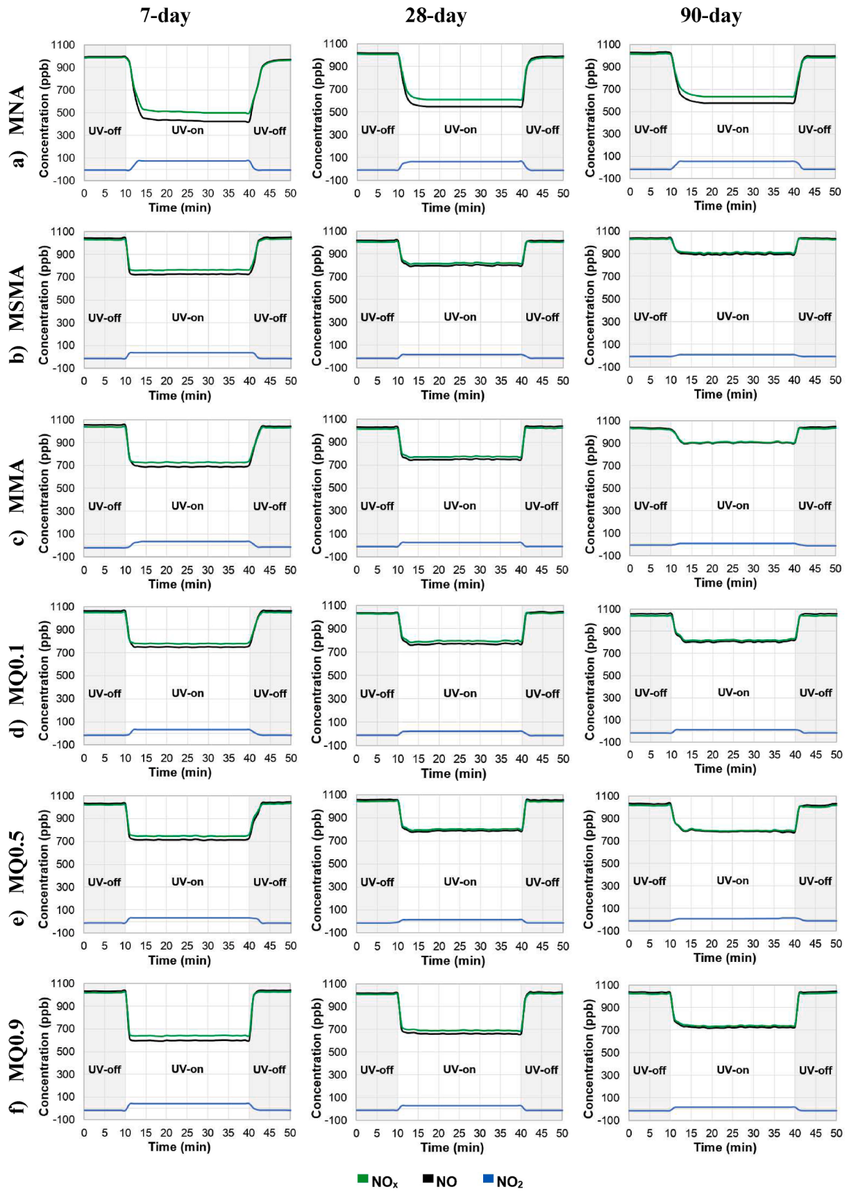
Fig. 8. Variation of \text{NO}_x , \text{NO} , and \text{NO}_2 concentration during each test for 7, 28, and 90 days old specimens.
