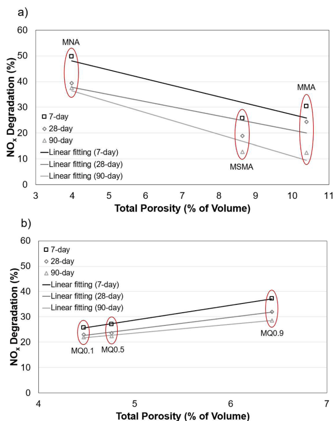
Fig. 14. Relationship between total porosity (% of volume) and \text{NO} degradation rate of specimens for (a) PSD non-optimized specimens (b) PSD optimized specimens.
