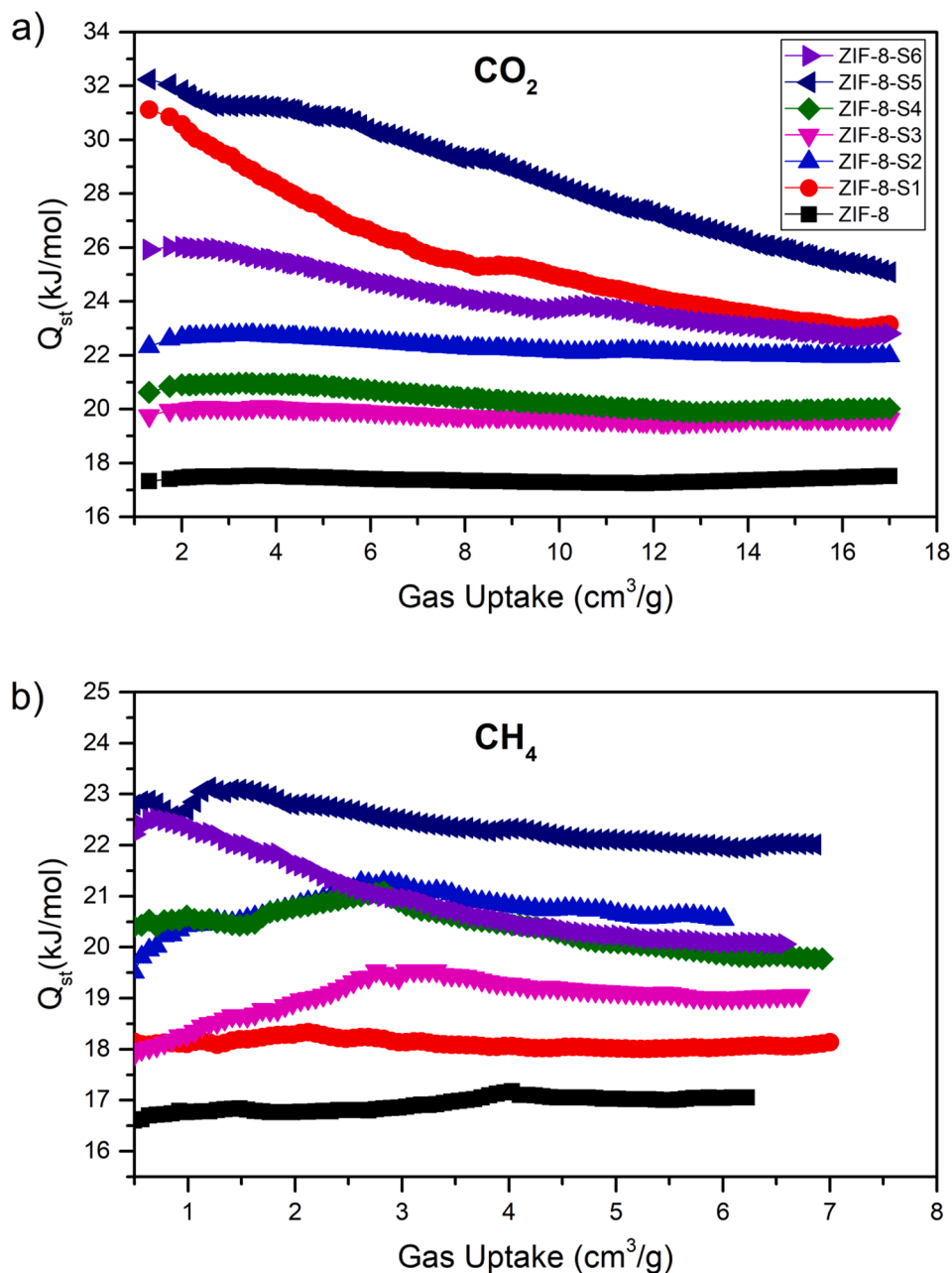
Fig. 3. Isothermic heats of adsorptions ( Q_{st} ) as a function of gas loading in \text{cm}^3 \text{g}^{-1} for (a) \text{CO}_2 and (b) \text{CH}_4 .
