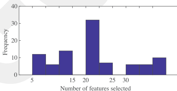
Figure 3. Histogram of the number of features selected on each training set of the leave-one-out cross-validation when no data normalization is performed.
