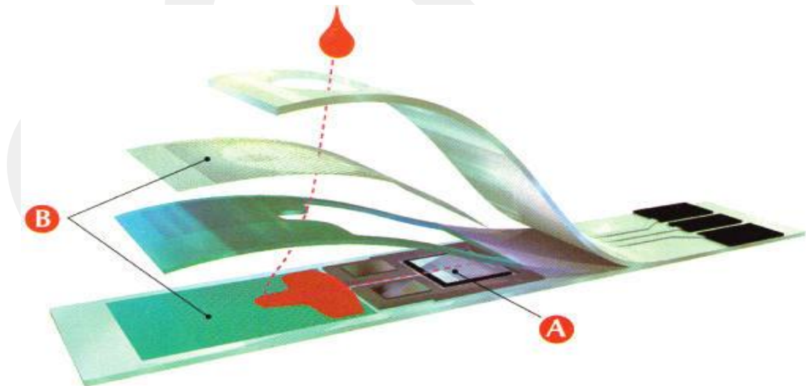
Figure 1.1.1.1: An example of a glucose measurement sensor (A) sensing part; (B) detecting part (drawing the blood). [4]
