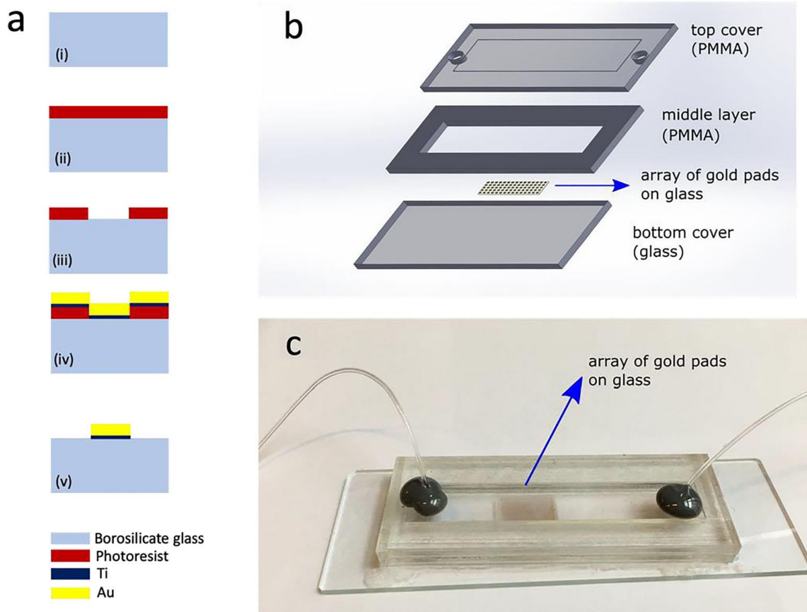
Figure 5.1.1.3: Fabrication process of the system (a) Microfabrication process flow for the array of gold pads: i) borosilicate glass wafer cleaning, (ii) spin coating of photoresist, (iii) patterning photoresist, (iv) titanium and gold deposition (v) lift-off process (b) An illustration of the microfluidic chip (c) The assembled device [80].
