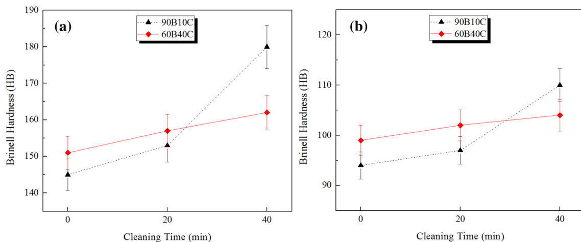
Fig. 8 Brinell hardness test results. a Cylindrical specimens and b prismatic specimens
