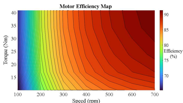
Fig. 11. Efficiency map of the optimized motor (up to 700 rpm)
