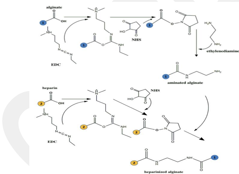
Figure 2.2.3.1 The mechanism of carbodiimide reactions for synthesize heparinized alginate
