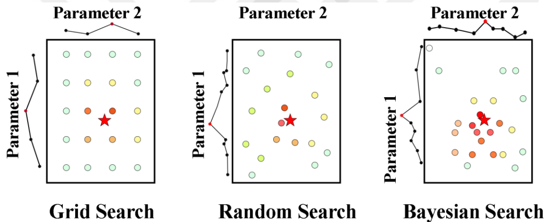
Figure 3.7 Illustration of grid, random and Bayesian search based hyperparameter optimization. The red star indicates the optimal parameter set.
