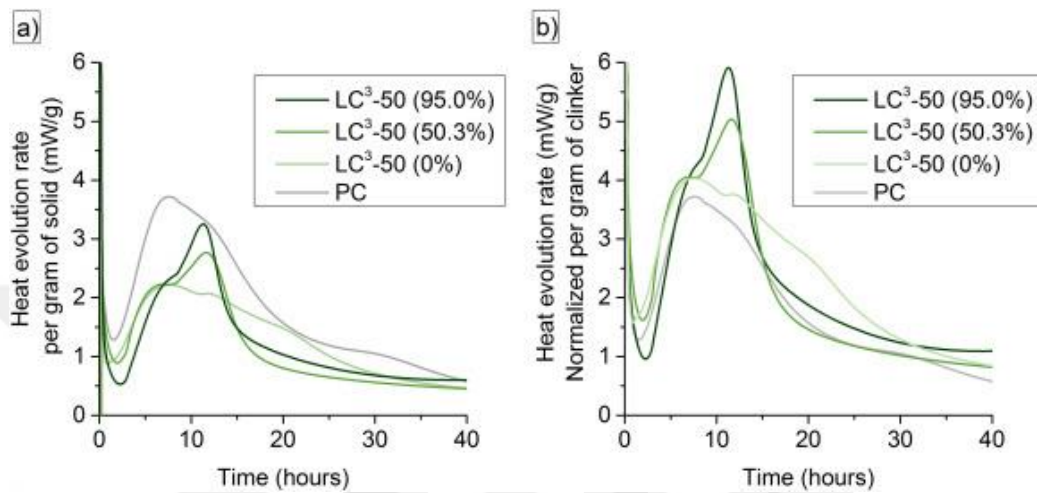
Figure 2.4.3 Heat release per gram of solid (a) and normalized per gram of clinker (b) [38]
