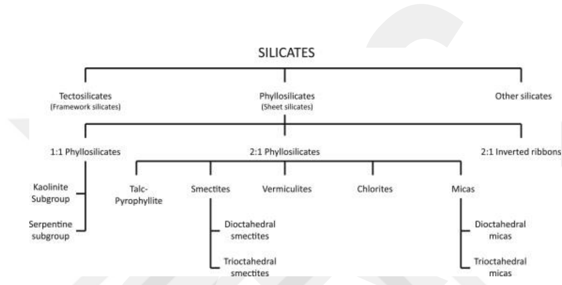
Figure 2.3.4.1 Classification of silicates with the main subgroups of clays [28]
