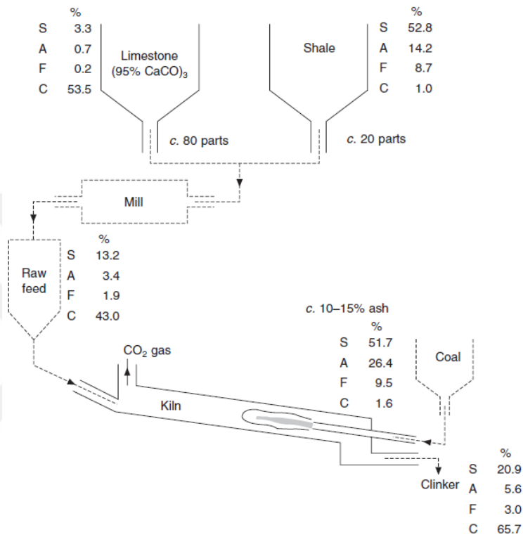
Figure 2.2.1.1 Clinker production analysis (S: SiO 2 , A: Al 2 O 3 , F: Fe 2 O 3 , C: CaO) [10]
